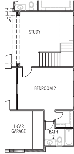
BONUS ROOM OPTION 2 WITH OPEN STUDY LOWER LEVEL
