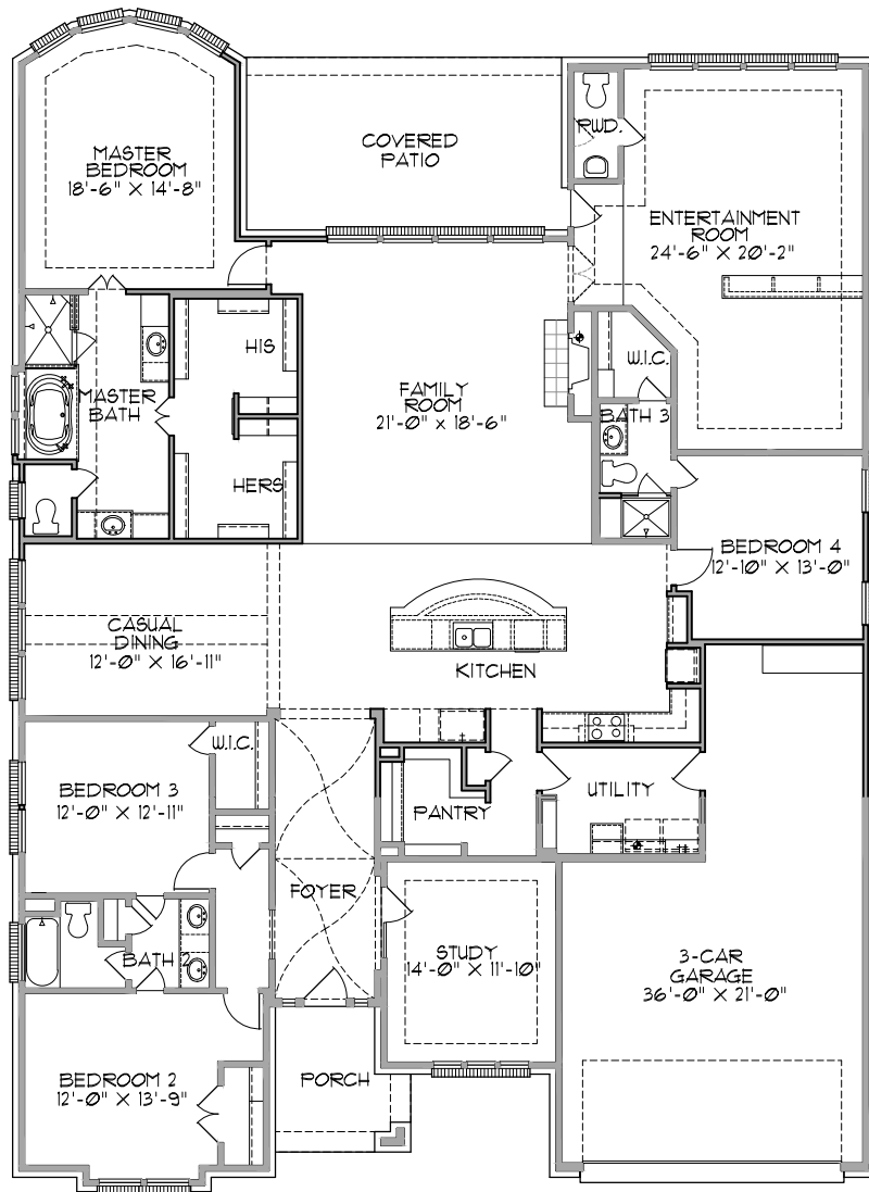
FIRST FLOOR
